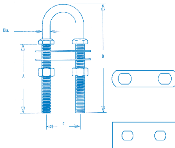
Typical Stern Eye Plate
